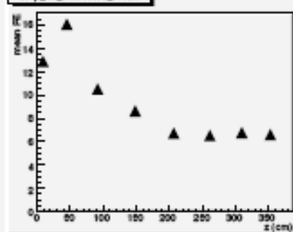
strip_46_truncated_mean
