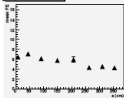
strip_41_truncated_mean
