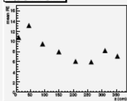
strip_47_truncated_mean
