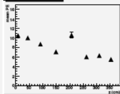
strip_40_truncated_mean
