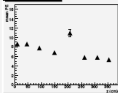
strip_38_truncated_mean
