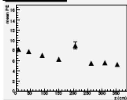
strip_37_truncated_mean
