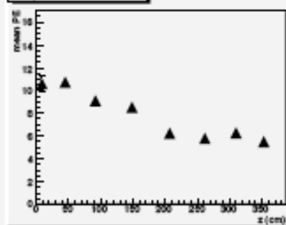
strip_42_truncated_mean
