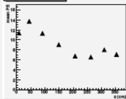
strip_44_truncated_mean
