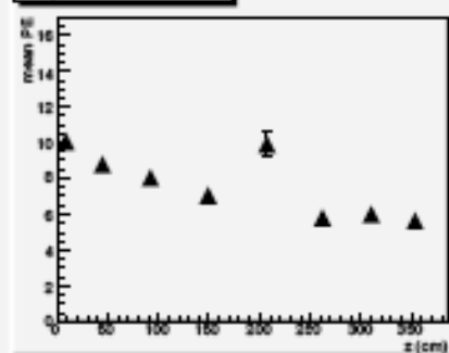
strip_39_truncated_mean
