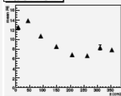
strip_48_truncated_mean
