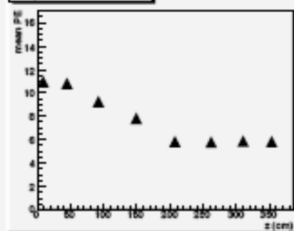
strip_43_truncated_mean
