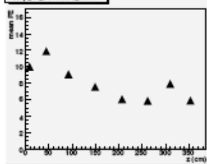
strip_45_truncated_mean
